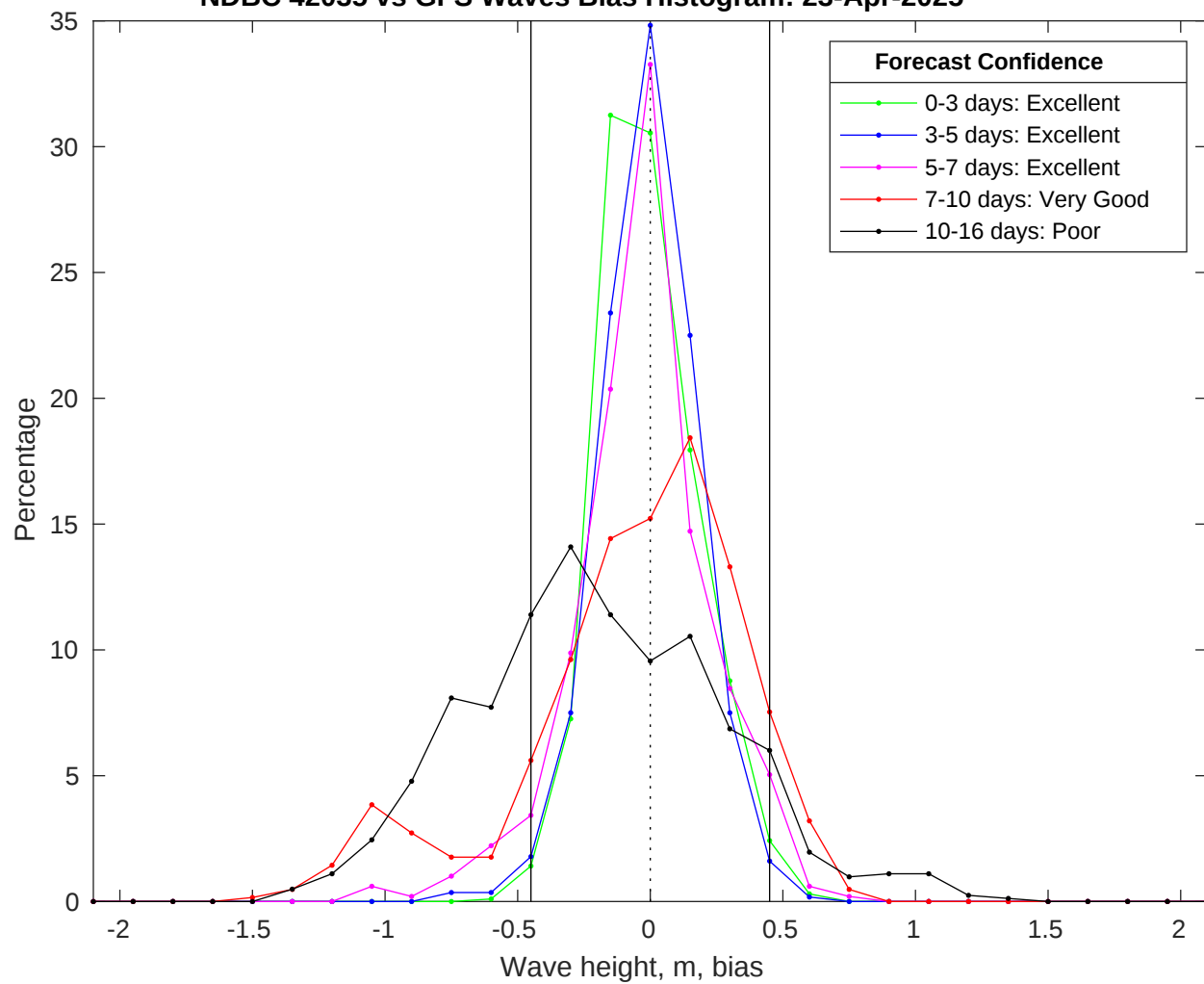
NDBC 42035 vs GFS Waves Bias Histogram: 23-Apr-2025
