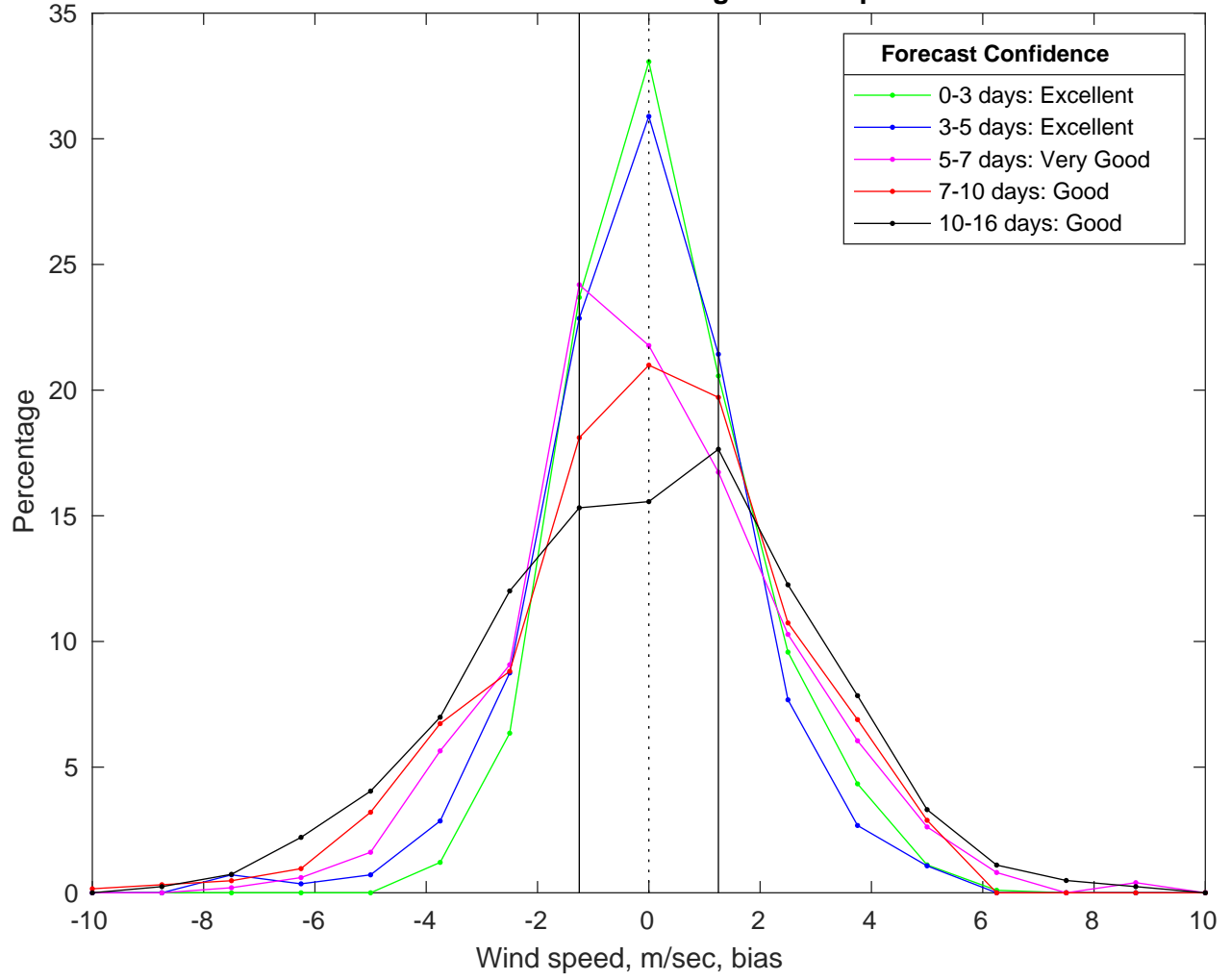
NDBC 42035 vs GFS Winds Bias Histogram: 23-Apr-2025
