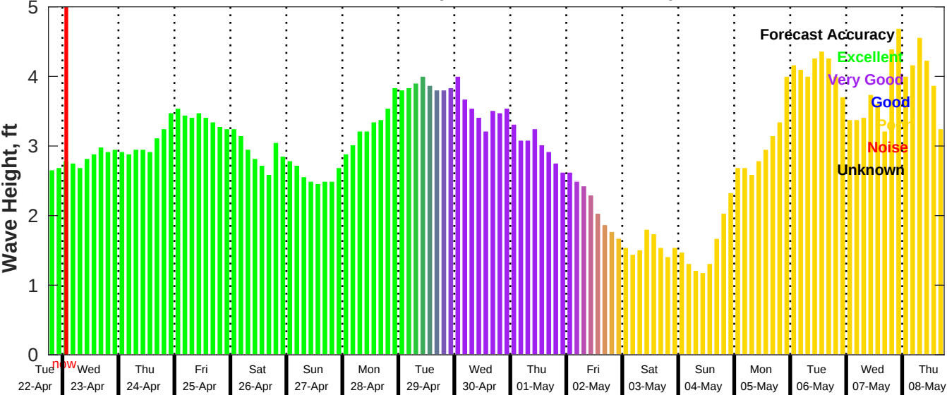
GFS Wave Forecast for NDBC 42035 from 22-Apr-2025 18:00:00 to 08-May-2025 18:00:00
