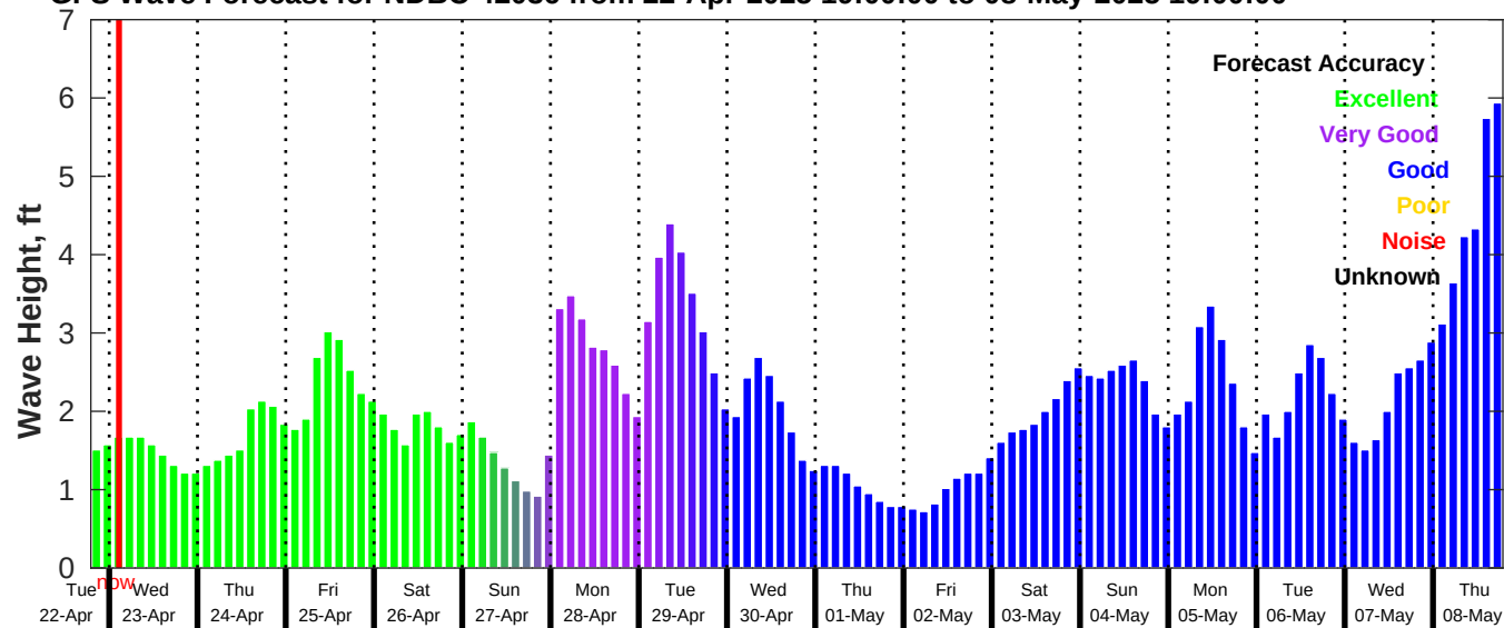
GFS Wave Forecast for NDBC 42036 from 22-Apr-2025 19:00:00 to 08-May-2025 19:00:00
