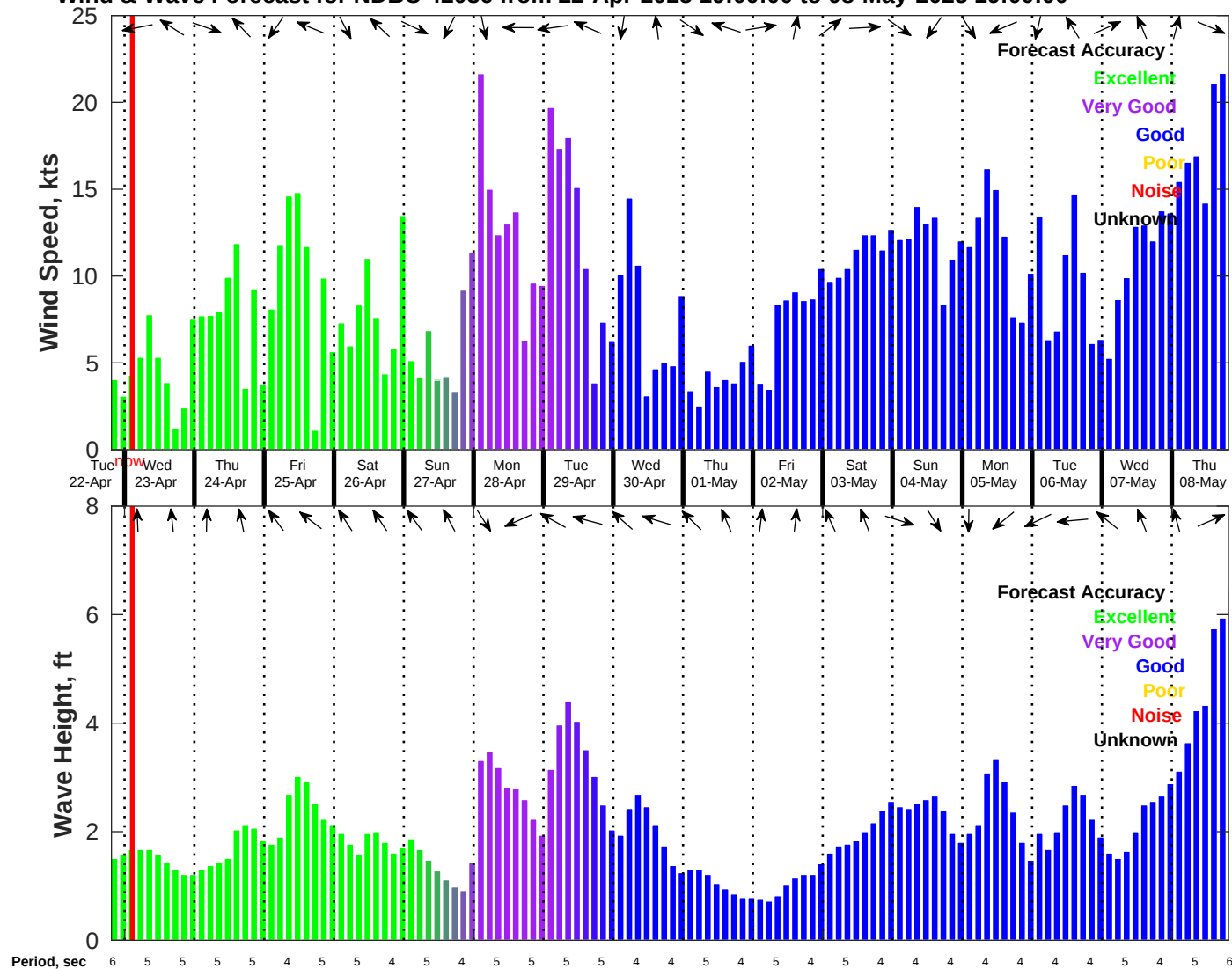
Wind & Wave Forecast for NDBC 42036 from 22-Apr-2025 19:00:00 to 08-May-2025 19:00:00
