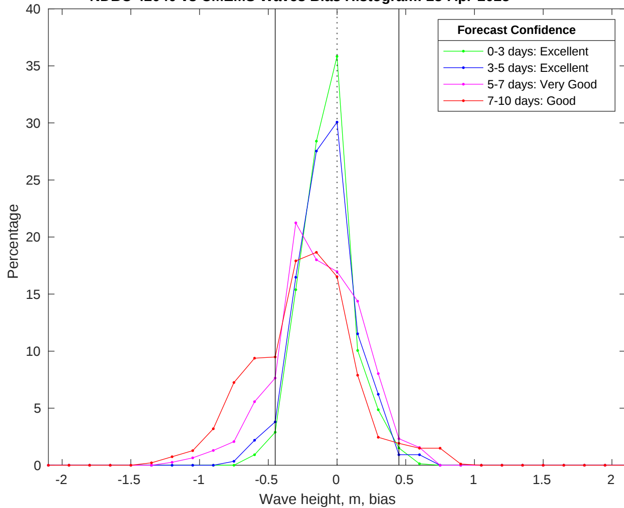
NDBC 42040 vs CMEMS Waves Bias Histogram: 23-Apr-2025
