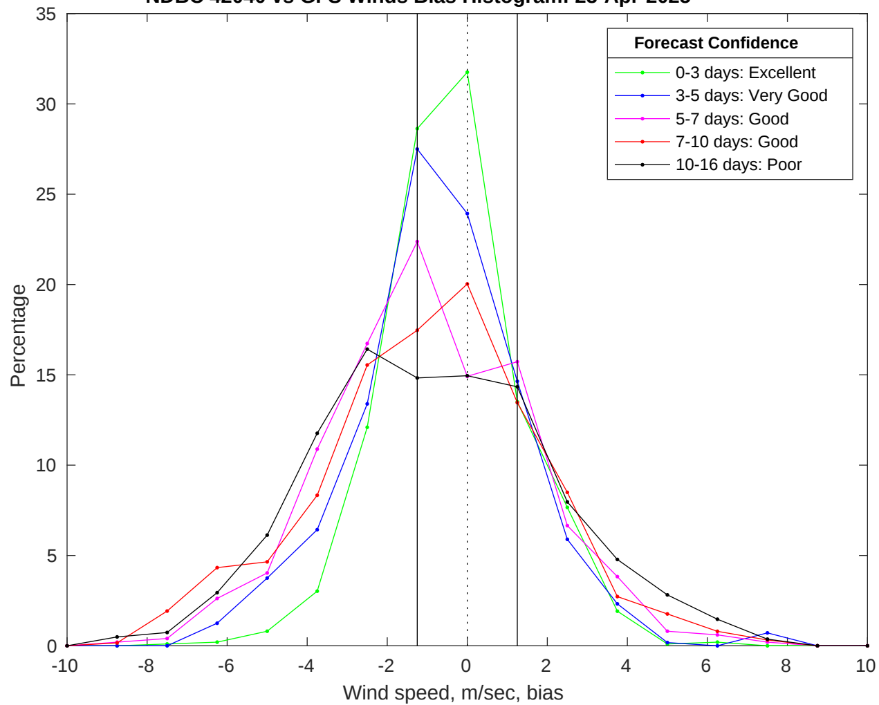
NDBC 42040 vs GFS Winds Bias Histogram: 23-Apr-2025
