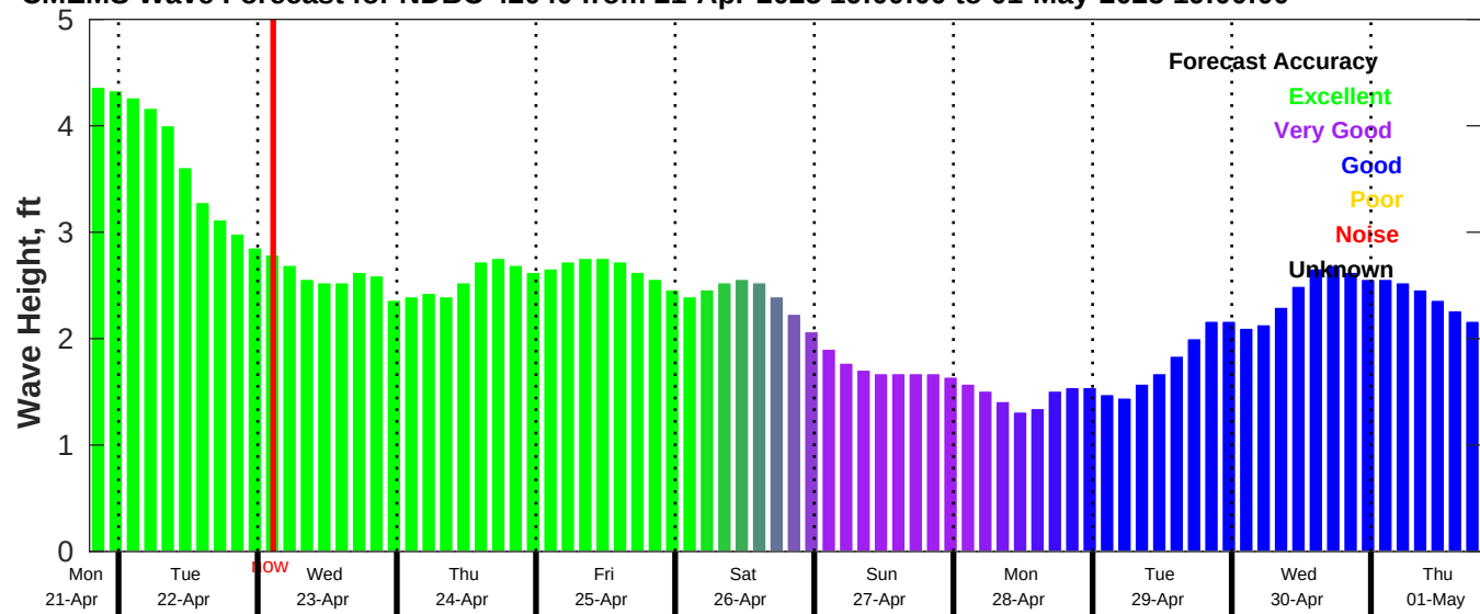
CMEMS Wave Forecast for NDBC 42040 from 21-Apr-2025 19:00:00 to 01-May-2025 19:00:00
