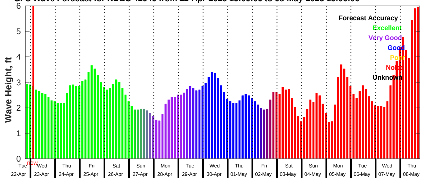
GFS Wave Forecast for NDBC 42040 from 22-Apr-2025 19:00:00 to 08-May-2025 19:00:00
