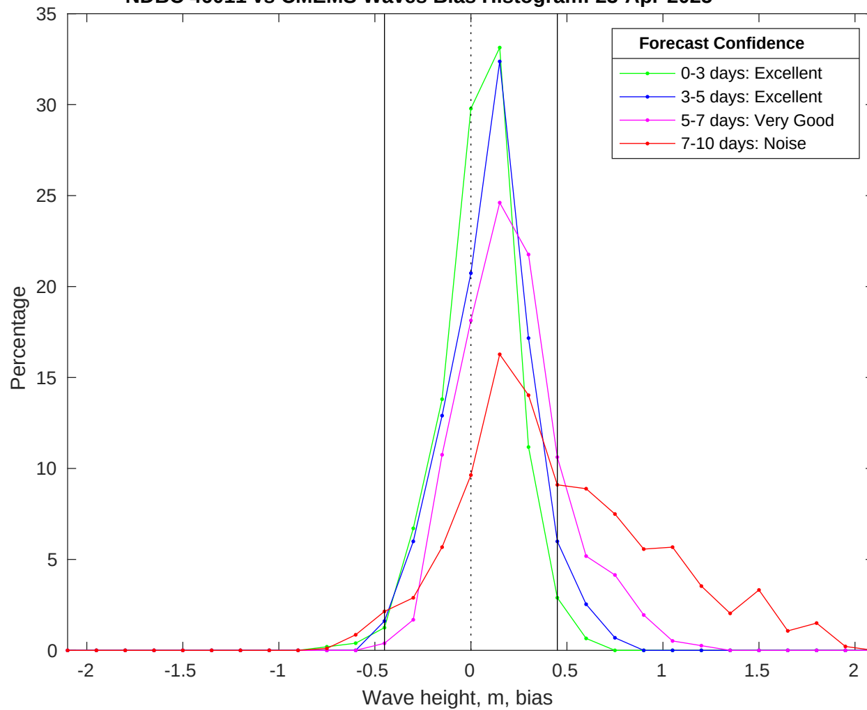
NDBC 46011 vs CMEMS Waves Bias Histogram: 23-Apr-2025
