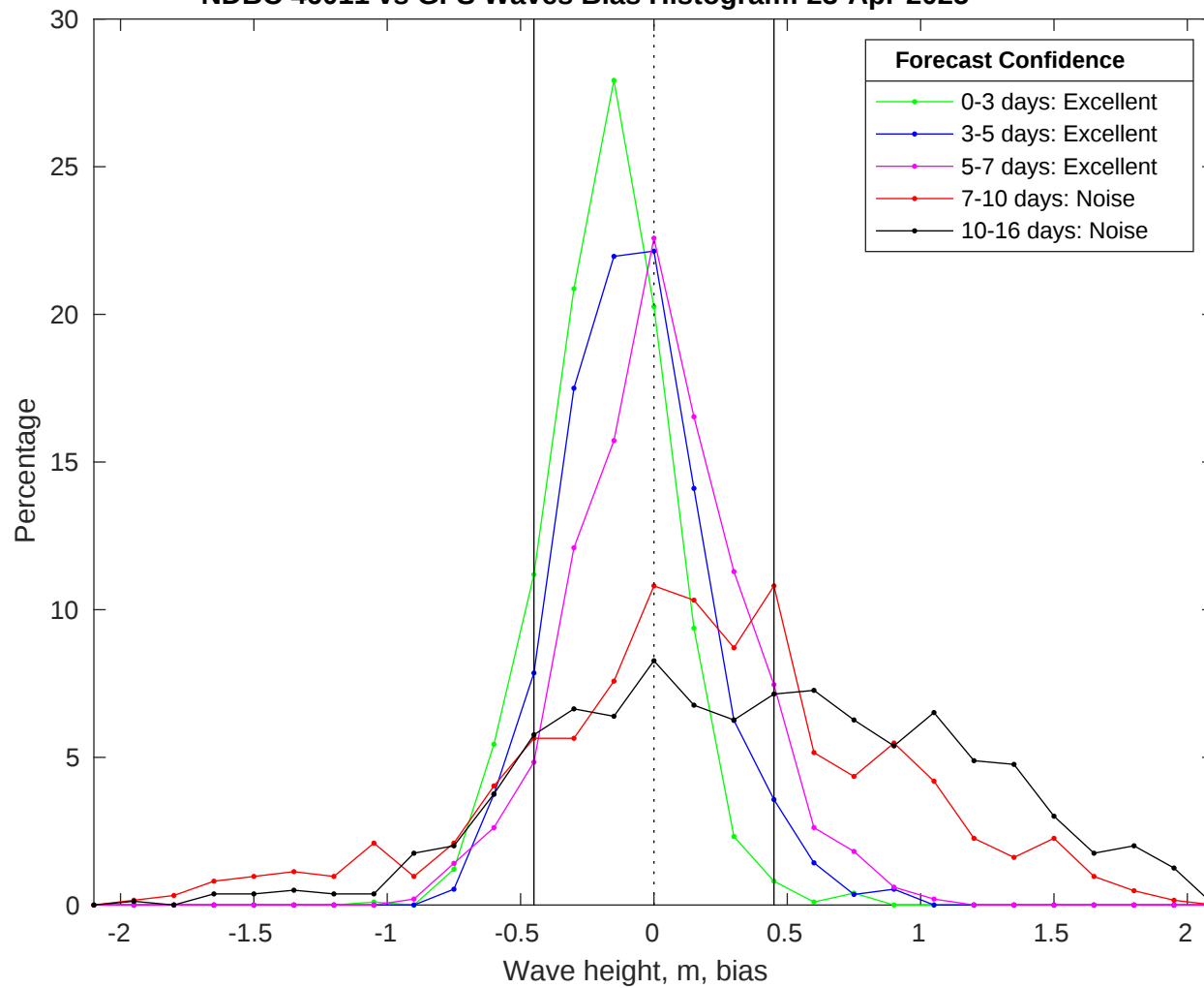
NDBC 46011 vs GFS Waves Bias Histogram: 23-Apr-2025
