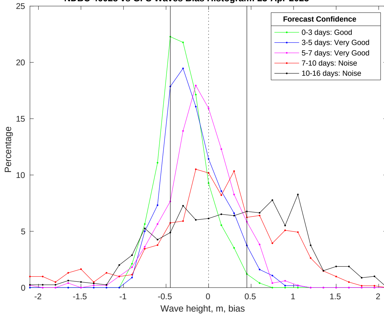
NDBC 46028 vs GFS Waves Bias Histogram: 23-Apr-2025
