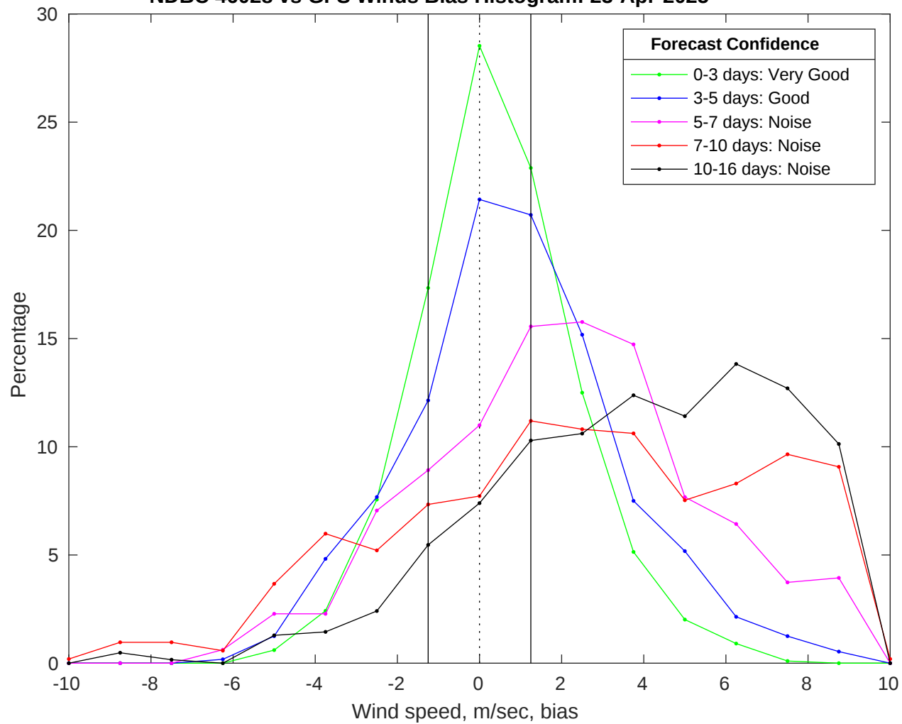
NDBC 46028 vs GFS Winds Bias Histogram: 23-Apr-2025
