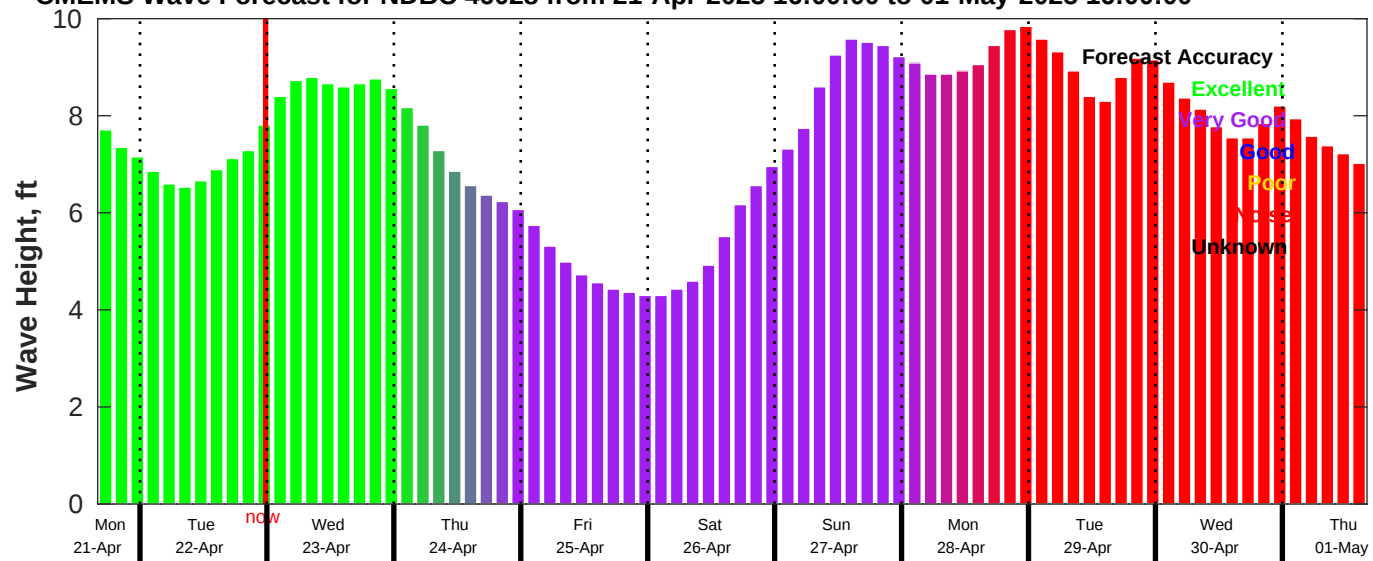
CMEMS Wave Forecast for NDBC 46028 from 21-Apr-2025 16:00:00 to 01-May-2025 16:00:00
