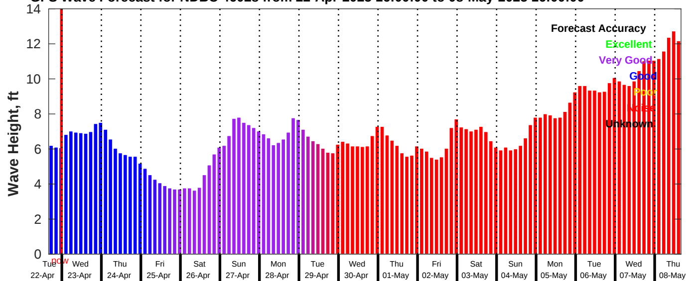
GFS Wave Forecast for NDBC 46028 from 22-Apr-2025 16:00:00 to 08-May-2025 16:00:00
