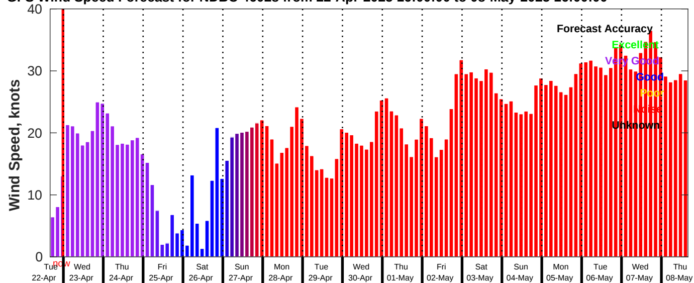
GFS Wind Speed Forecast for NDBC 46028 from 22-Apr-2025 16:00:00 to 08-May-2025 16:00:00
