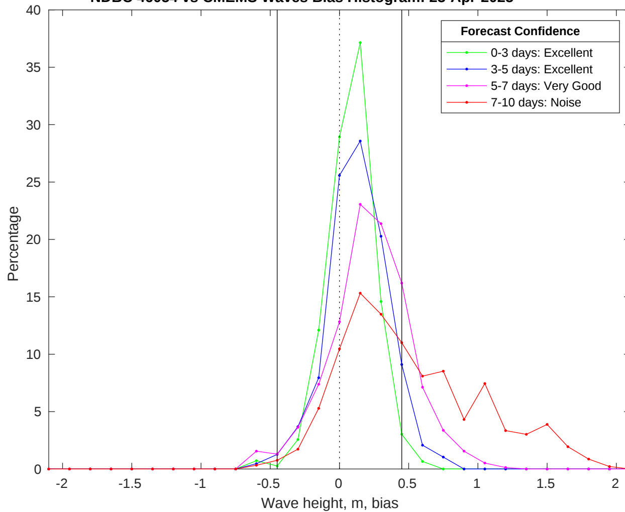
NDBC 46054 vs CMEMS Waves Bias Histogram: 23-Apr-2025
