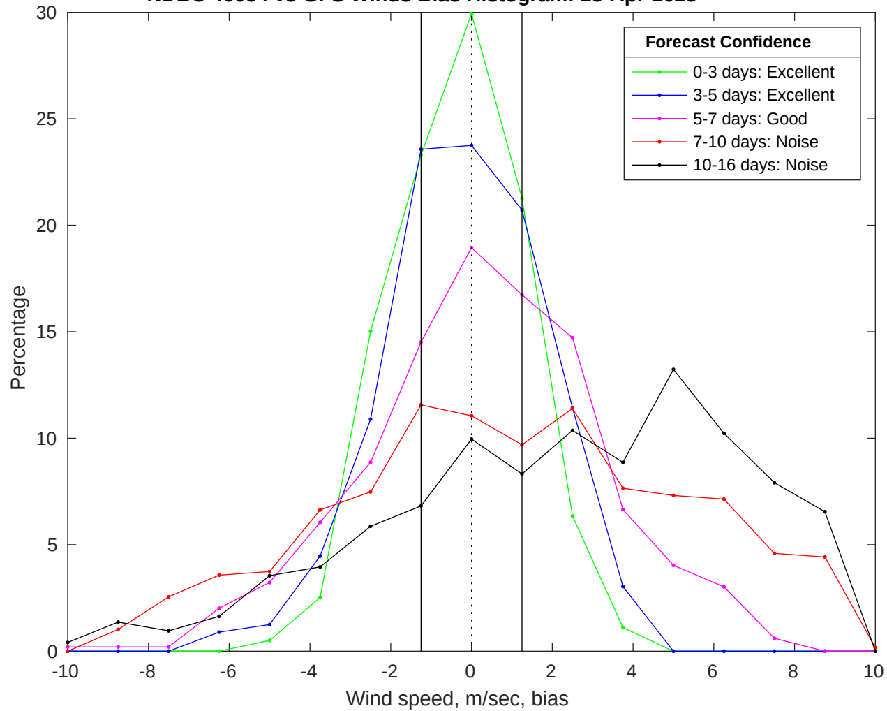
NDBC 46054 vs GFS Winds Bias Histogram: 23-Apr-2025
