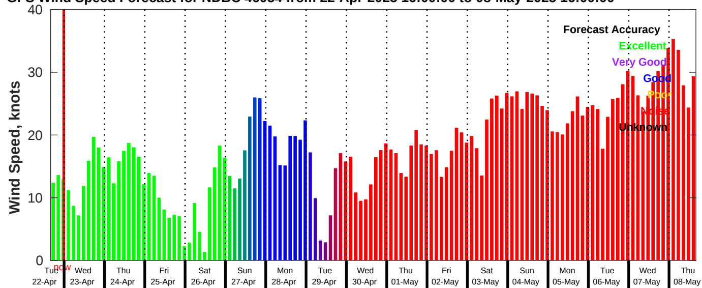
GFS Wind Speed Forecast for NDBC 46054 from 22-Apr-2025 16:00:00 to 08-May-2025 16:00:00
