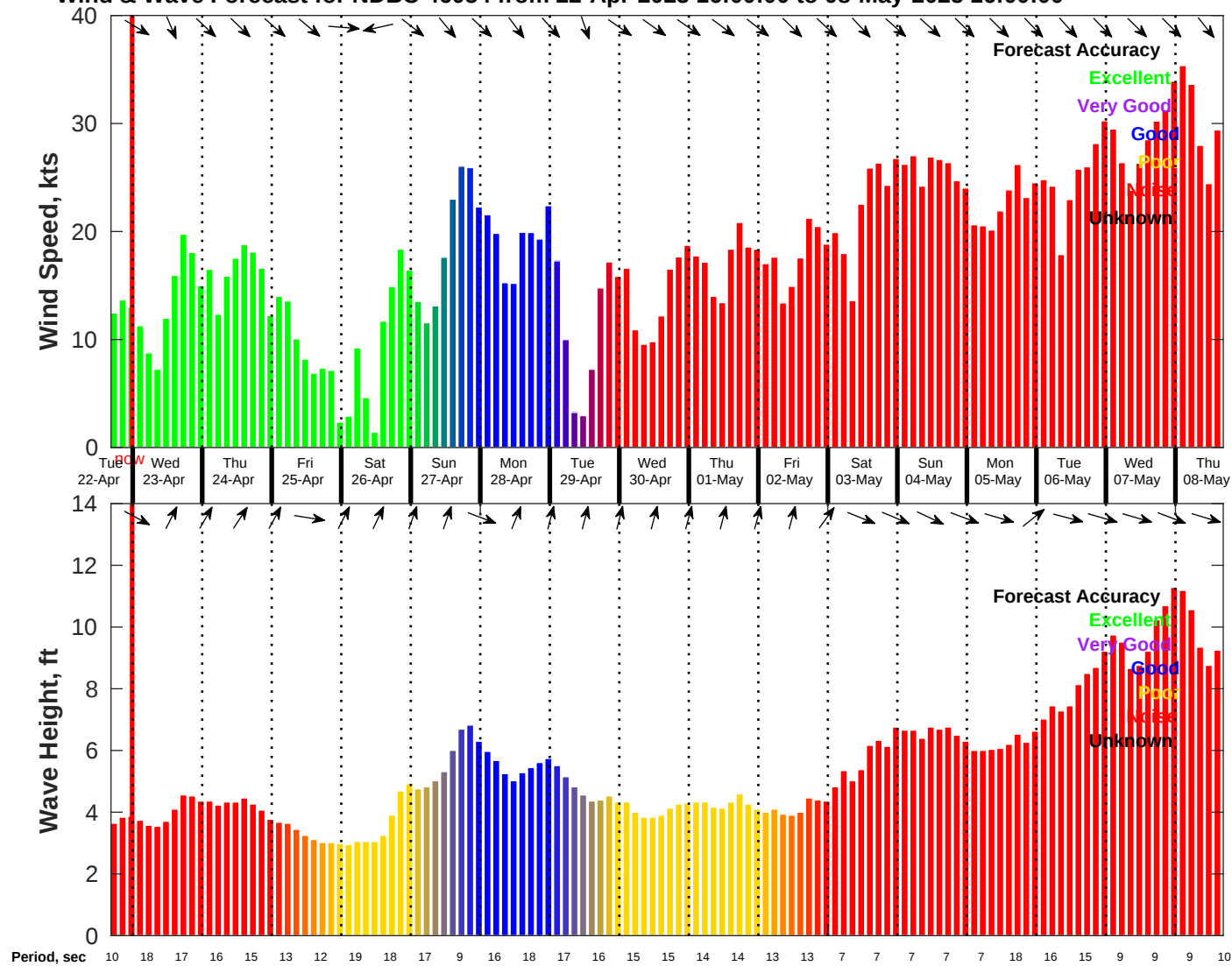
Wind & Wave Forecast for NDBC 46054 from 22-Apr-2025 16:00:00 to 08-May-2025 16:00:00
