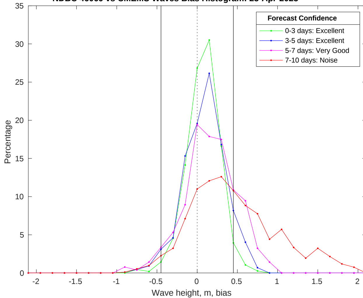
NDBC 46069 vs CMEMS Waves Bias Histogram: 23-Apr-2025
