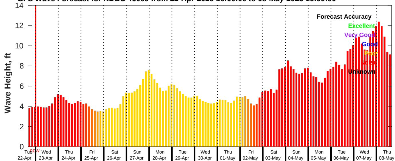
GFS Wave Forecast for NDBC 46069 from 22-Apr-2025 16:00:00 to 08-May-2025 16:00:00
