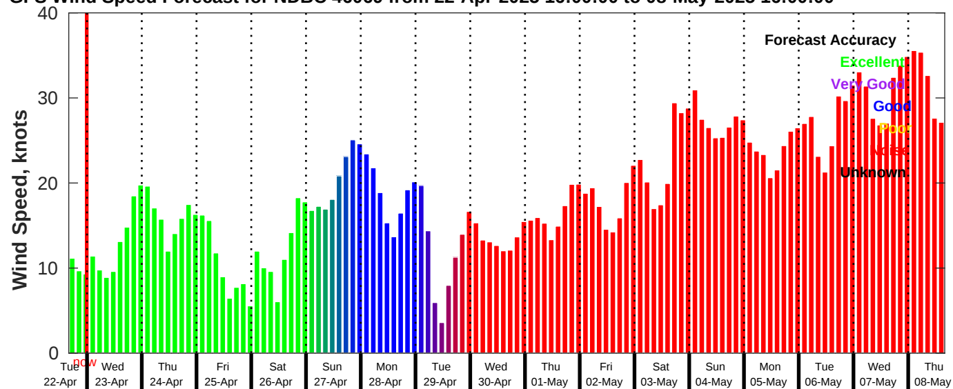
GFS Wind Speed Forecast for NDBC 46069 from 22-Apr-2025 16:00:00 to 08-May-2025 16:00:00
