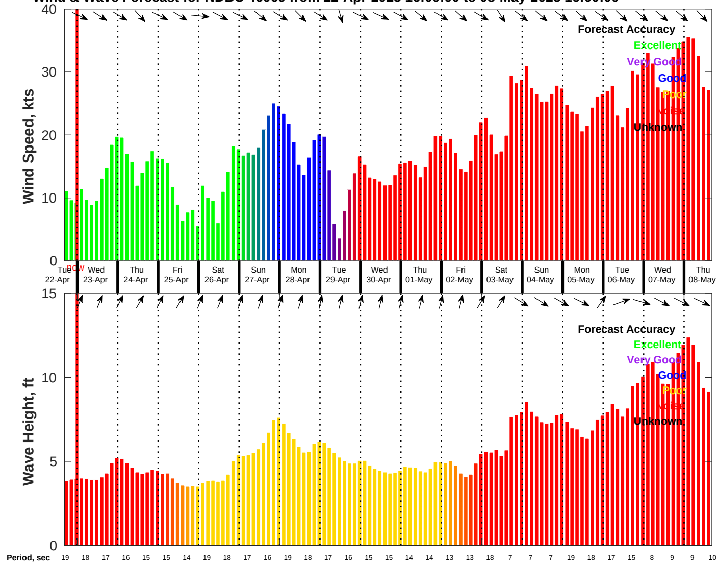
Wind & Wave Forecast for NDBC 46069 from 22-Apr-2025 16:00:00 to 08-May-2025 16:00:00
