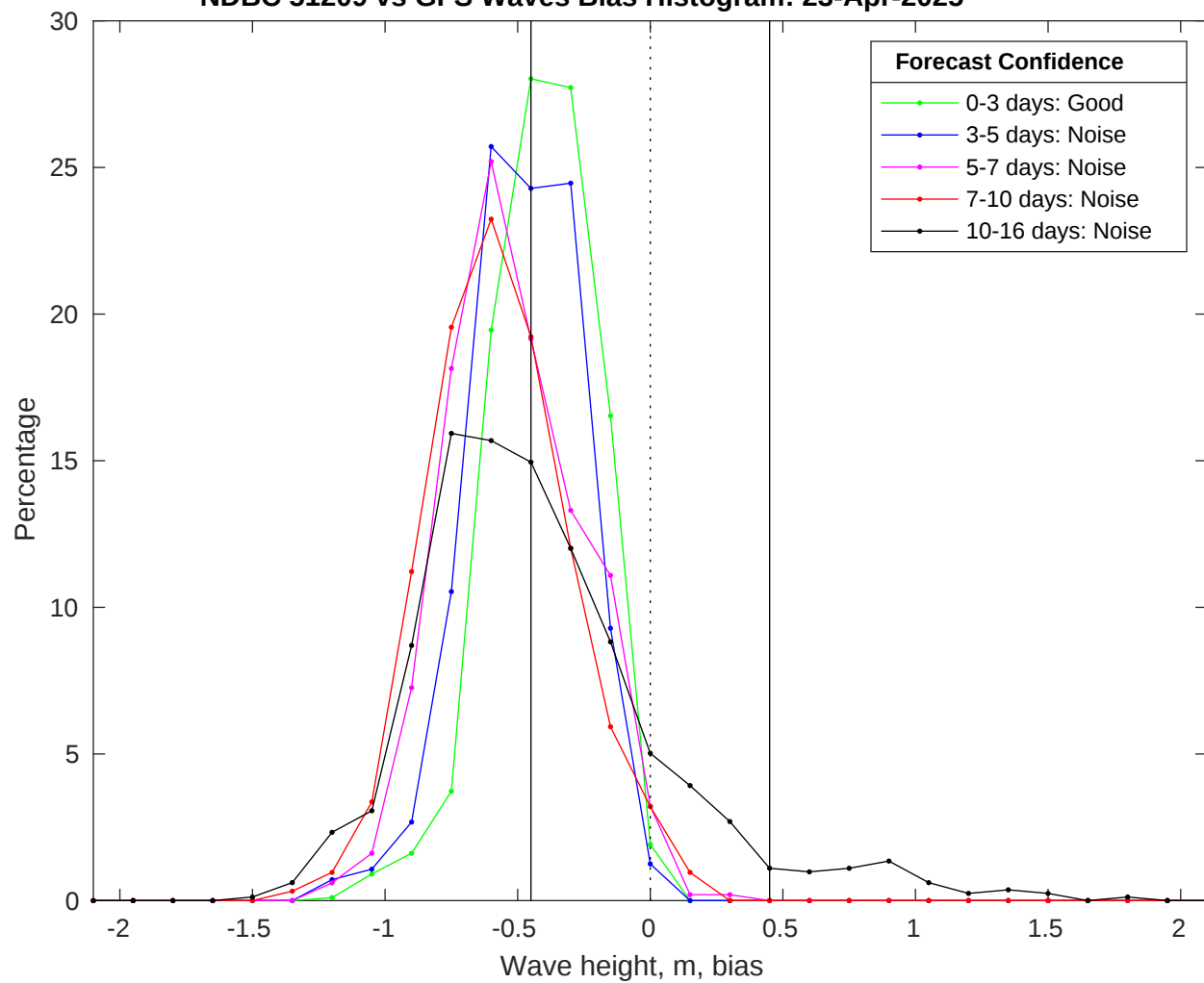
NDBC 51209 vs GFS Waves Bias Histogram: 23-Apr-2025
