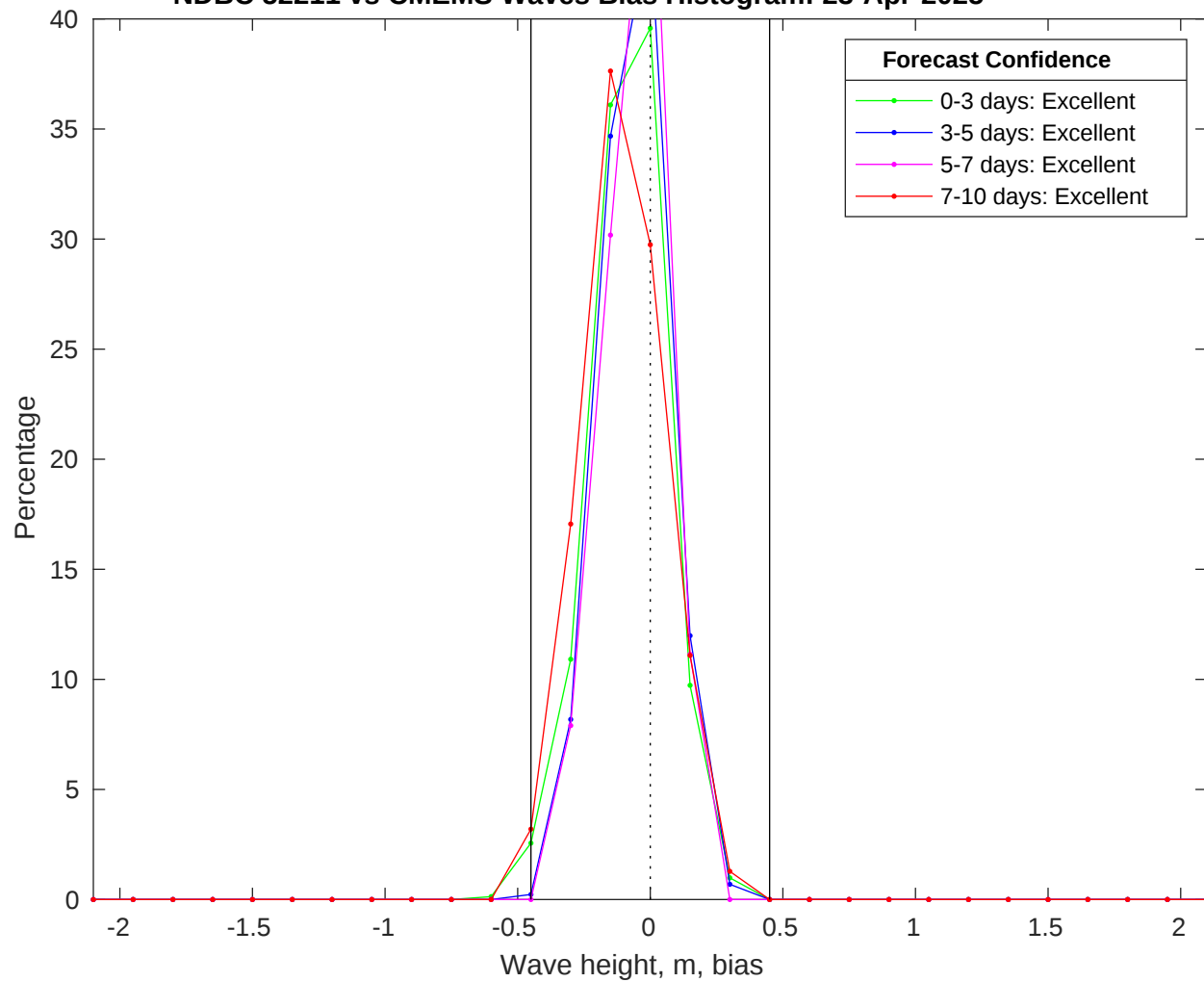
NDBC 52211 vs CMEMS Waves Bias Histogram: 23-Apr-2025
