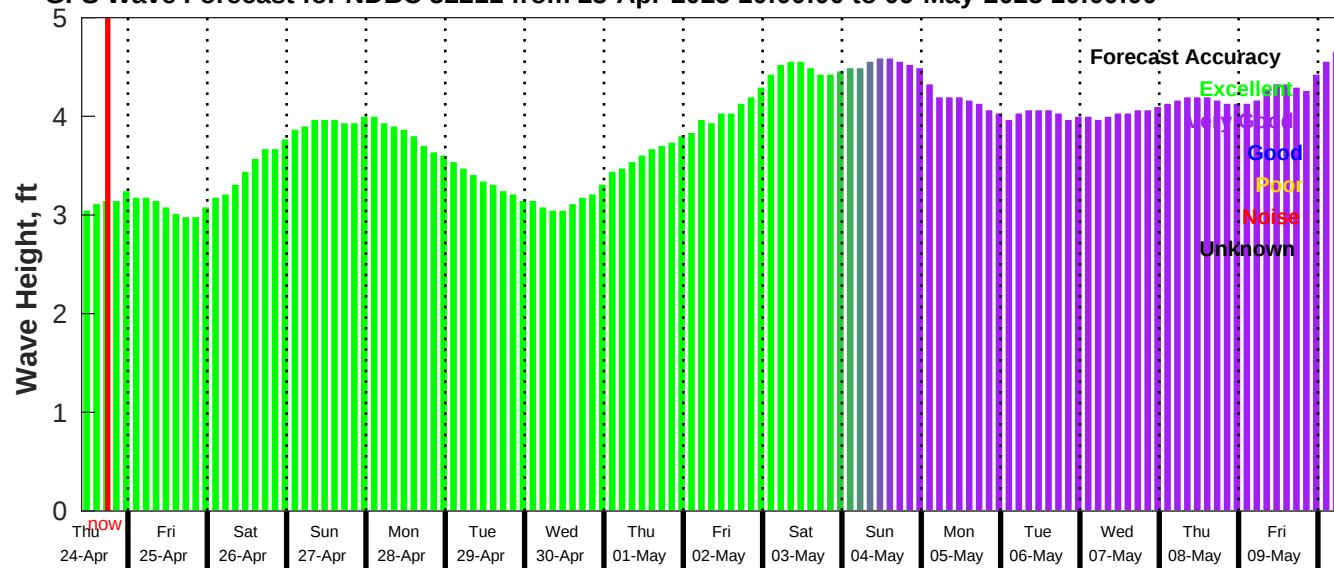
GFS Wave Forecast for NDBC 52211 from 23-Apr-2025 10:00:00 to 09-May-2025 10:00:00
