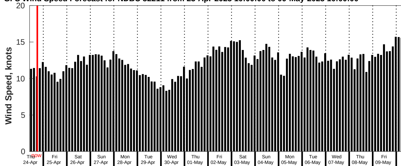
GFS Wind Speed Forecast for NDBC 52211 from 23-Apr-2025 10:00:00 to 09-May-2025 10:00:00
