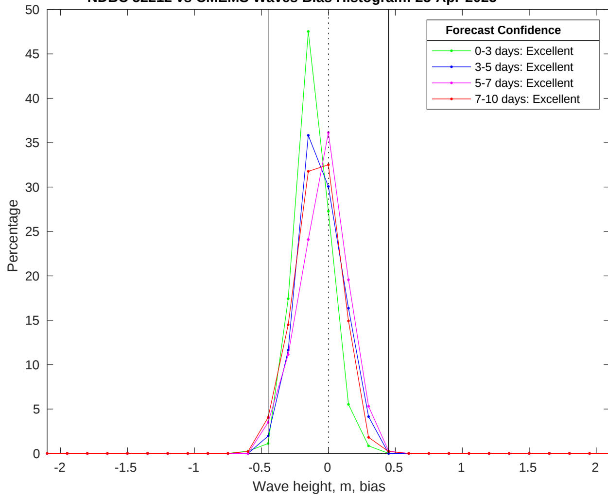
NDBC 52212 vs CMEMS Waves Bias Histogram: 23-Apr-2025
