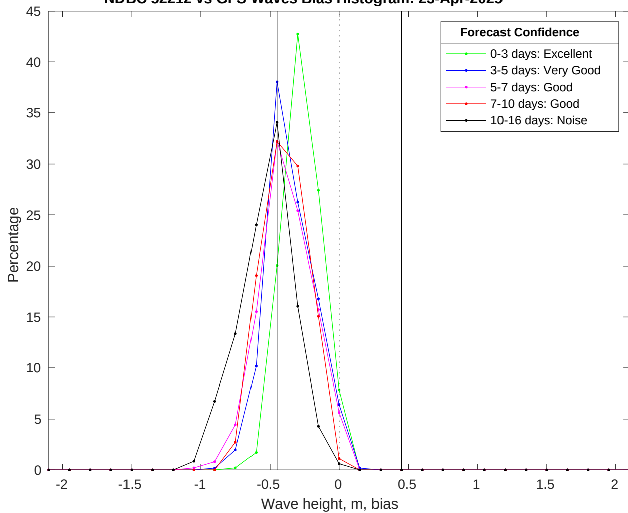
NDBC 52212 vs GFS Waves Bias Histogram: 23-Apr-2025
