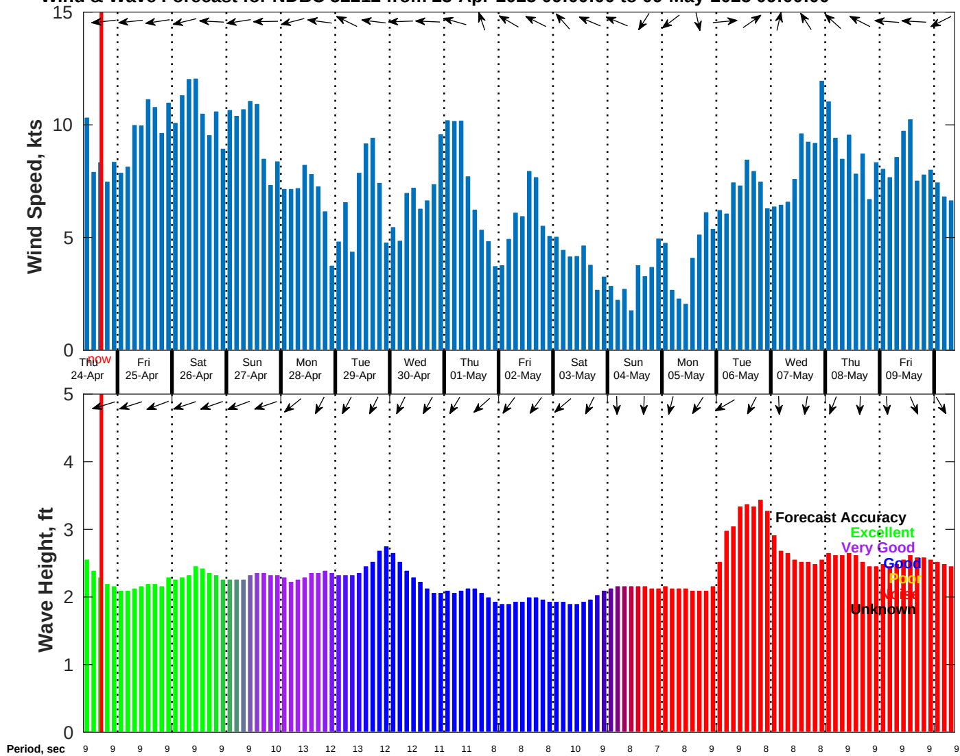
Wind & Wave Forecast for NDBC 52212 from 23-Apr-2025 09:00:00 to 09-May-2025 09:00:00
