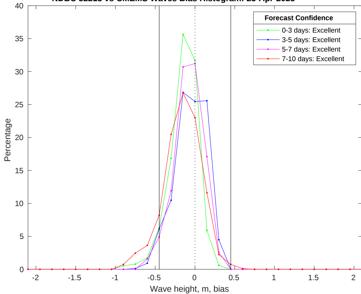
NDBC 52213 vs CMEMS Waves Bias Histogram: 23-Apr-2025
