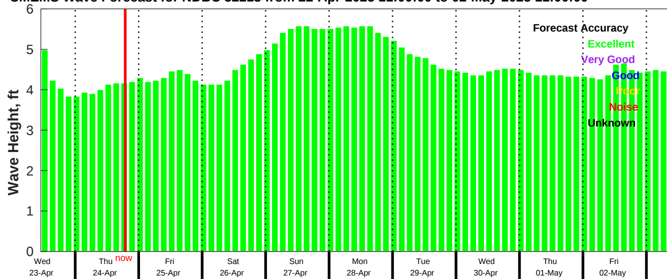
CMEMS Wave Forecast for NDBC 52213 from 22-Apr-2025 11:00:00 to 02-May-2025 11:00:00
