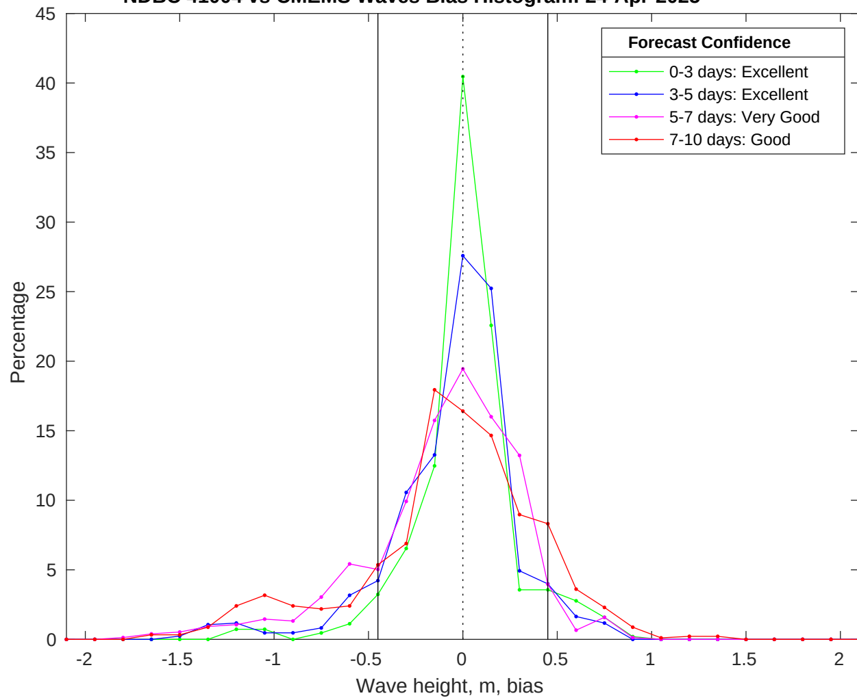
NDBC 41004 vs CMEMS Waves Bias Histogram: 24-Apr-2025
