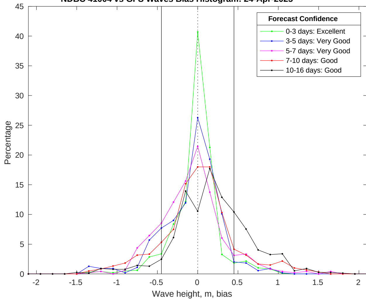
NDBC 41004 vs GFS Waves Bias Histogram: 24-Apr-2025
