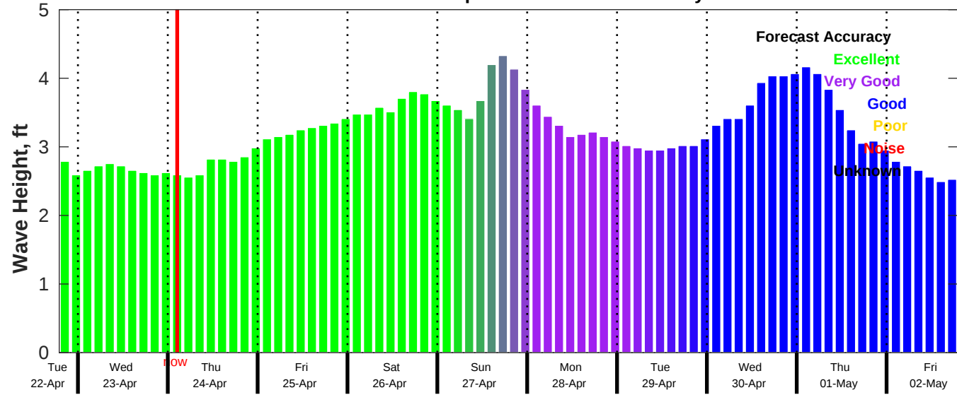
CMEMS Wave Forecast for NDBC 41004 from 22-Apr-2025 19:00:00 to 02-May-2025 19:00:00
