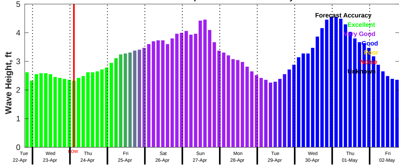
CMEMS Wave Forecast for NDBC 41013 from 22-Apr-2025 19:00:00 to 02-May-2025 19:00:00
