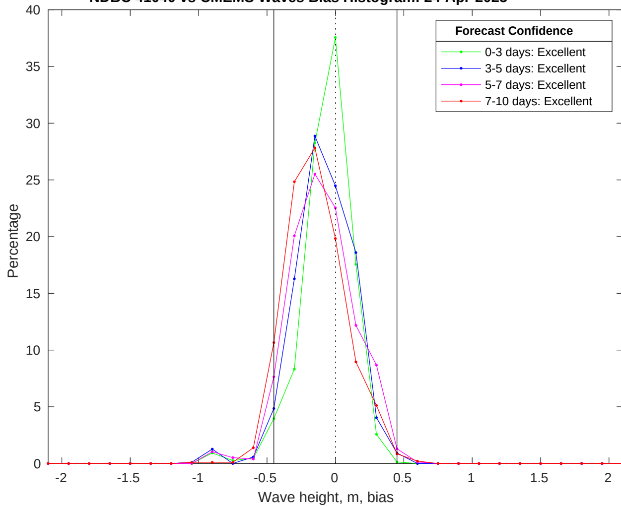
NDBC 41040 vs CMEMS Waves Bias Histogram: 24-Apr-2025
