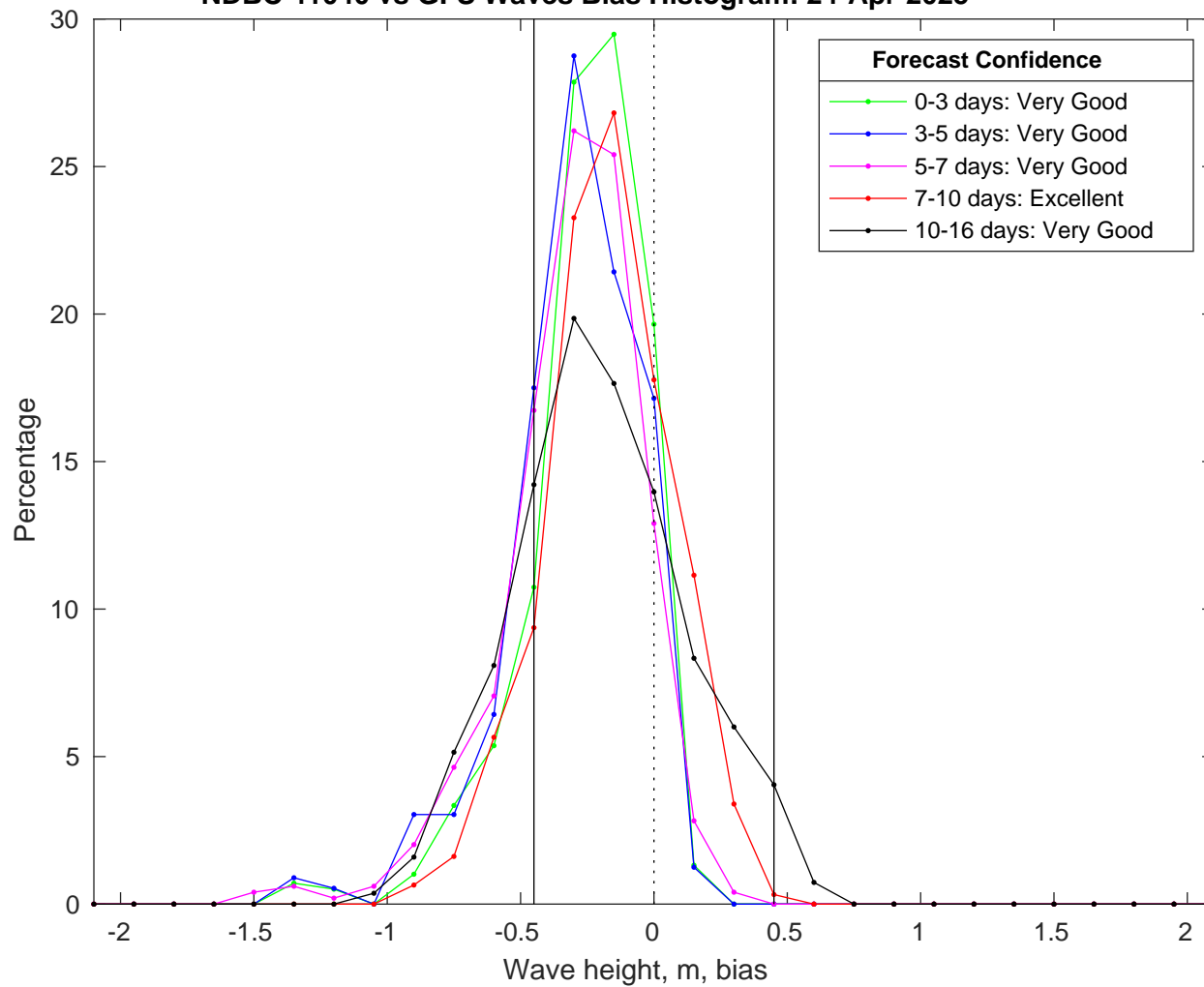
NDBC 41040 vs GFS Waves Bias Histogram: 24-Apr-2025
