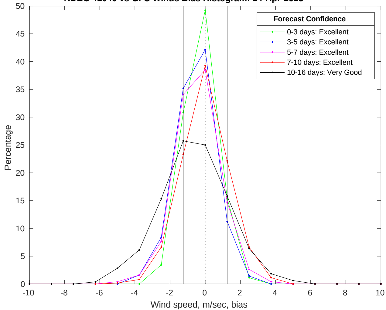
NDBC 41040 vs GFS Winds Bias Histogram: 24-Apr-2025
