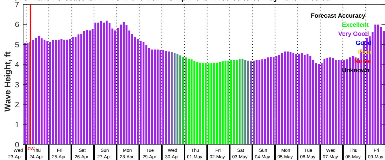
GFS Wave Forecast for NDBC 41040 from 23-Apr-2025 21:00:00 to 09-May-2025 21:00:00
