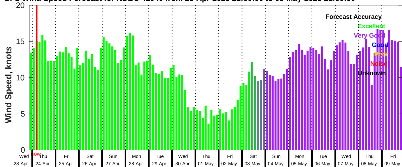
GFS Wind Speed Forecast for NDBC 41040 from 23-Apr-2025 21:00:00 to 09-May-2025 21:00:00
