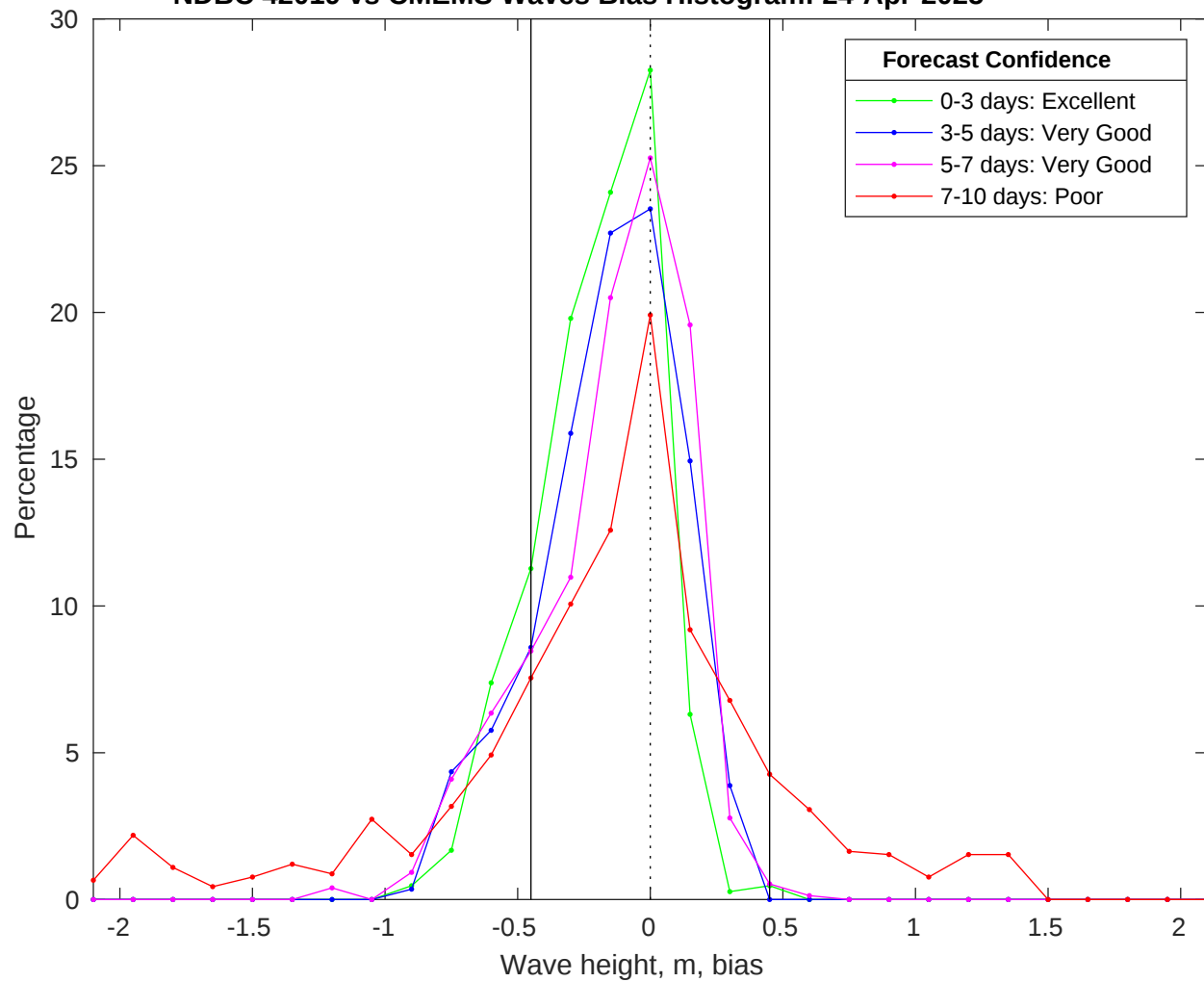
NDBC 42019 vs CMEMS Waves Bias Histogram: 24-Apr-2025
