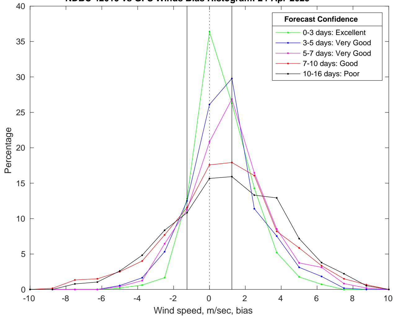
NDBC 42019 vs GFS Winds Bias Histogram: 24-Apr-2025
