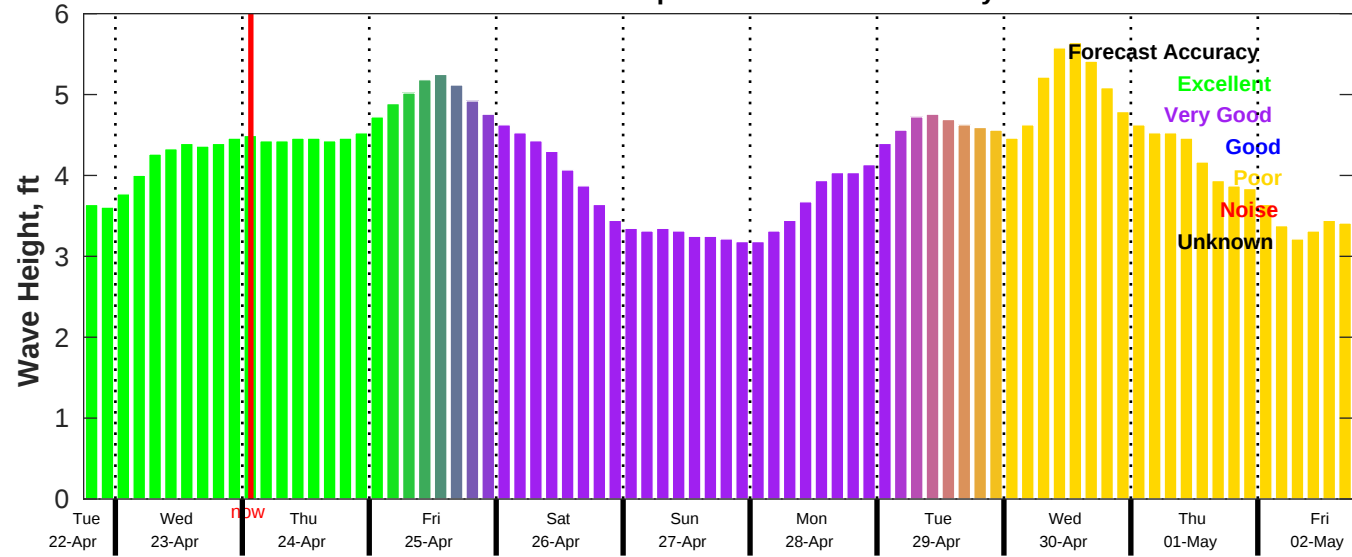
CMEMS Wave Forecast for NDBC 42019 from 22-Apr-2025 18:00:00 to 02-May-2025 18:00:00
