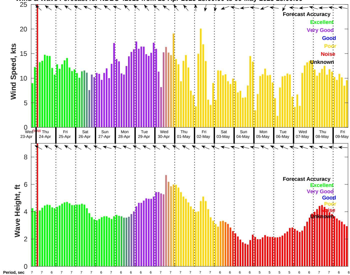
Wind & Wave Forecast for NDBC 42019 from 23-Apr-2025 18:00:00 to 09-May-2025 18:00:00
