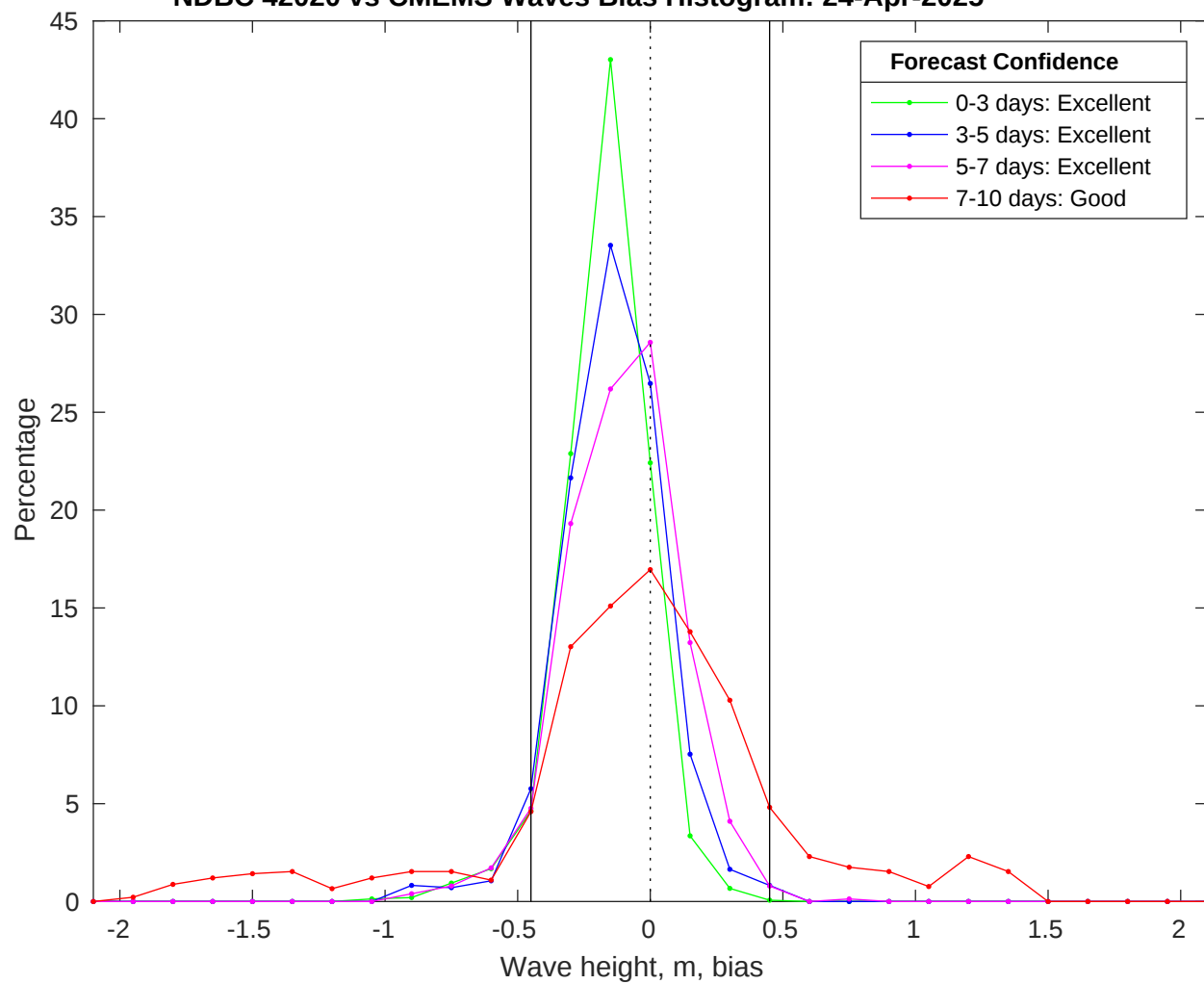
NDBC 42020 vs CMEMS Waves Bias Histogram: 24-Apr-2025
