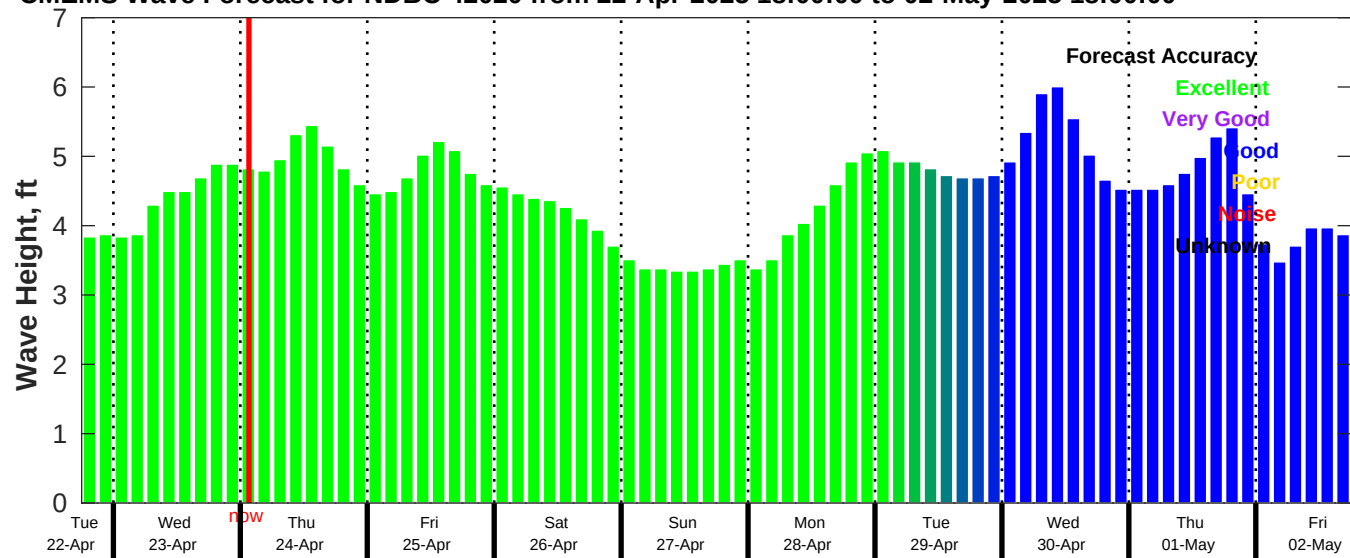
CMEMS Wave Forecast for NDBC 42020 from 22-Apr-2025 18:00:00 to 02-May-2025 18:00:00
