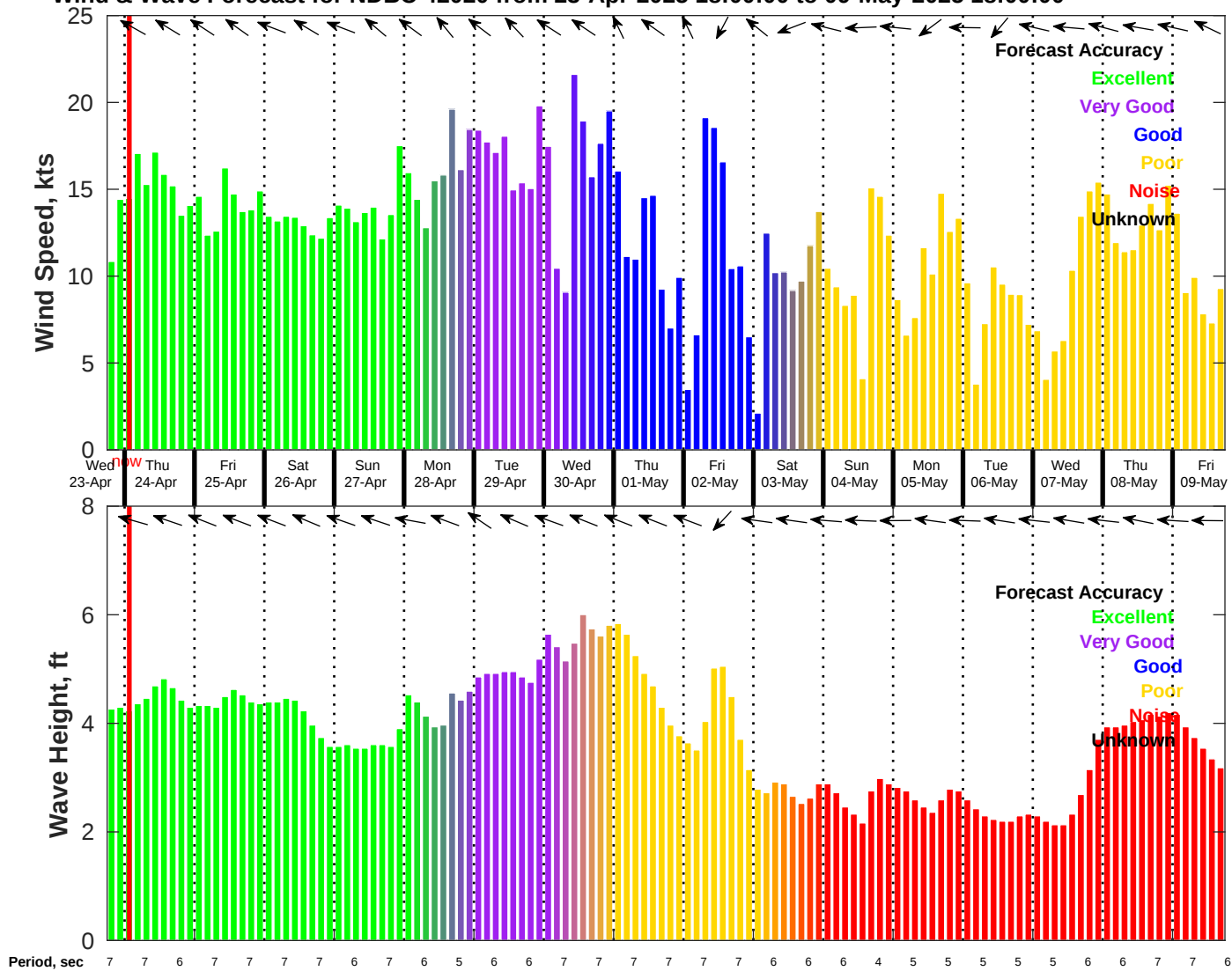
Wind & Wave Forecast for NDBC 42020 from 23-Apr-2025 18:00:00 to 09-May-2025 18:00:00
