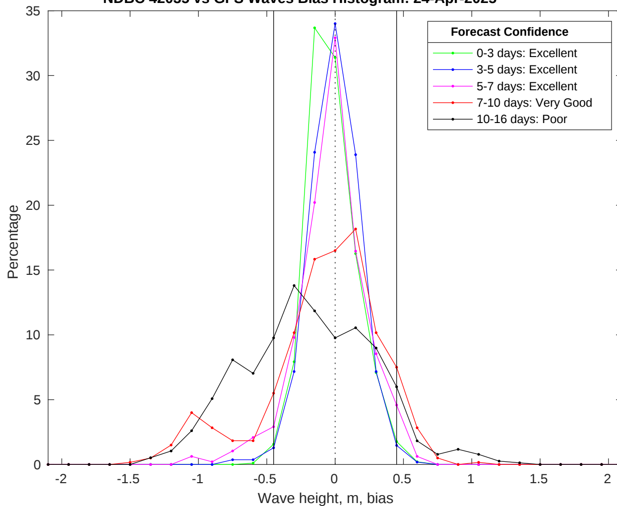
NDBC 42035 vs GFS Waves Bias Histogram: 24-Apr-2025
